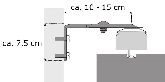
Wandmontage
