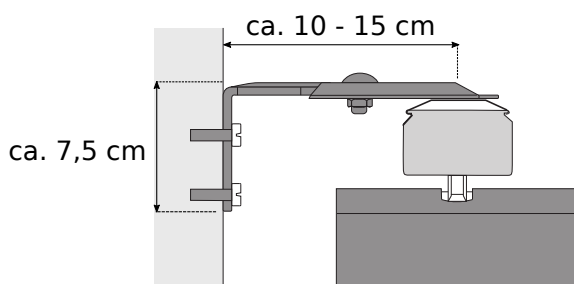
Wandmontage
